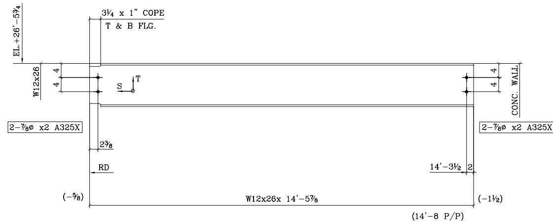
ONE - BEAM - D25D (GRID.NR.G/NR.3)
