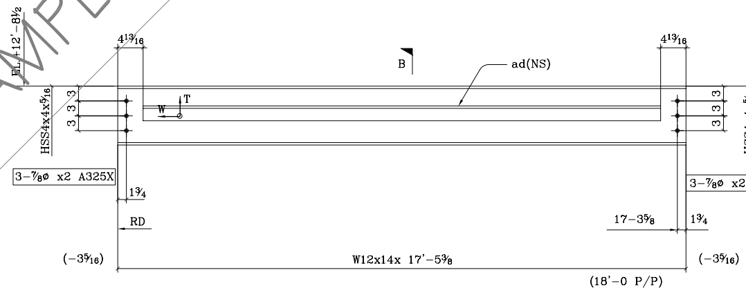
ONE - BEAM - D25F (GRID.2/BET.E-F)
